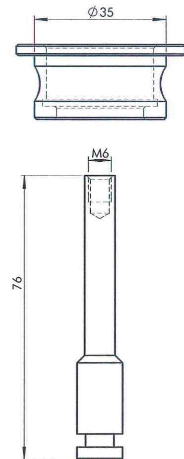
HONEYWELL ML
