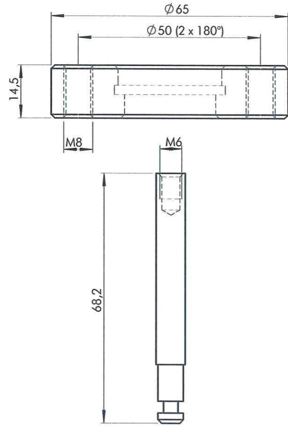
TAHC MC55/100
