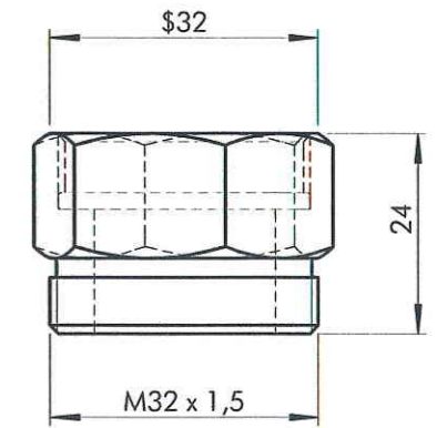
SAMSON 5825
